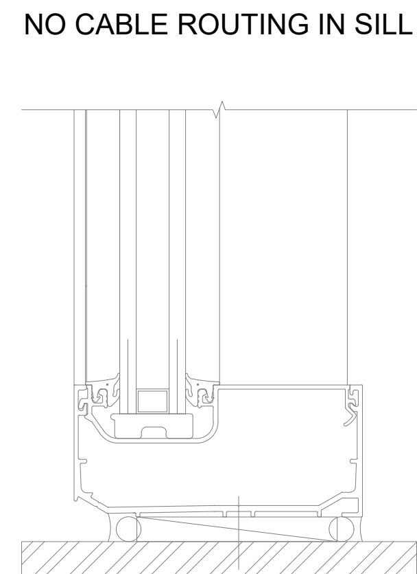
DETAIL 3 SILL
