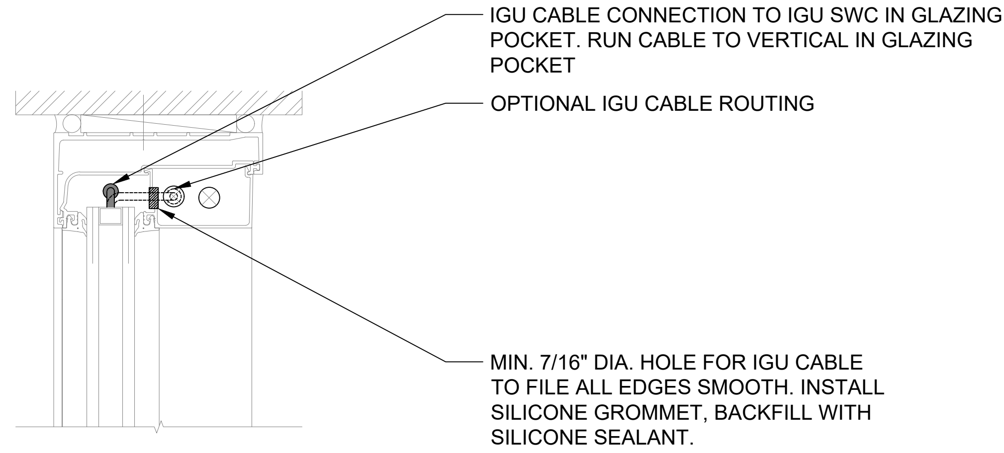
DETAIL 1 HEAD
