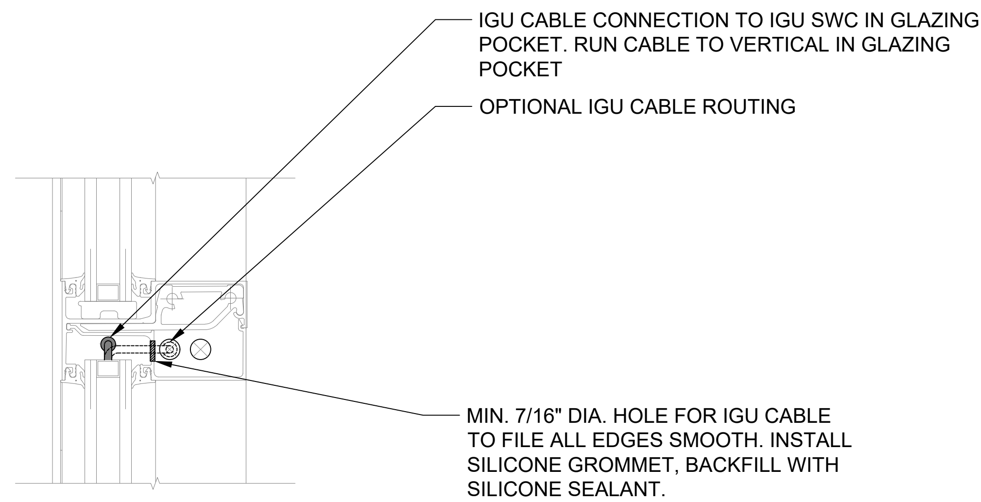
DETAIL 1 HEAD
